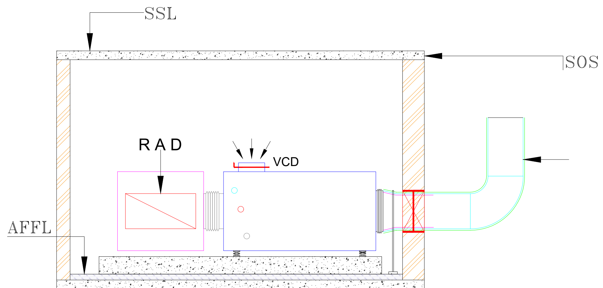
AHU05 SECTION DRAWING
